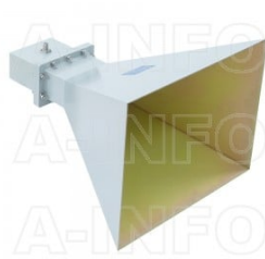
LB-650-15-C-NF Standard Gain Horn Antenna 1.12-1.7GHz 15dB Gain N Type Female
